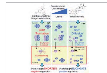
Schematic model of BSS1/BOP1 function in brassinosteroid signaling
