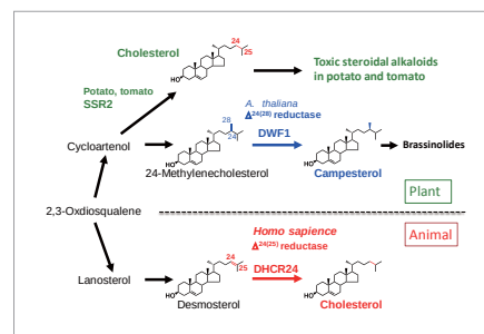
Biosynthesis of steroids in plant and animal. SSR2 gene responsible for biosynthesis of toxic steroidal glycoalkaloids in potato was identified
